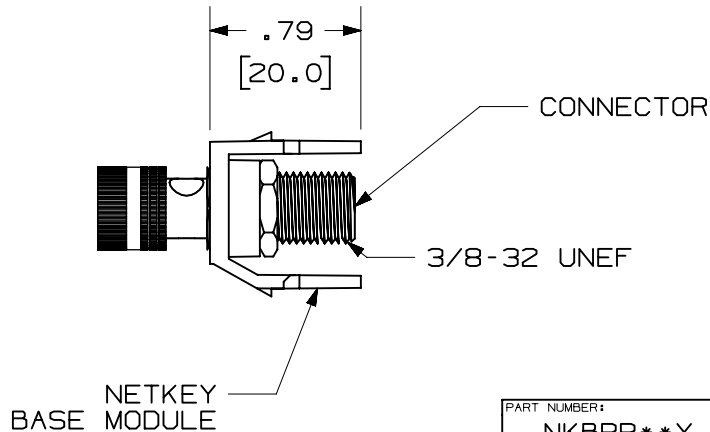
KNURLED NUT WITH COLOR BAND
