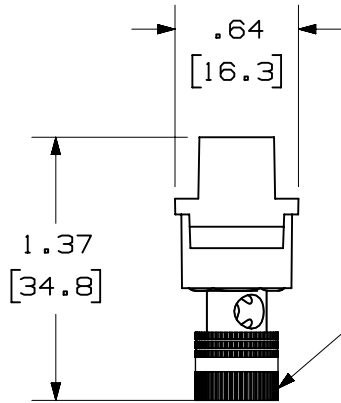
KNURLED NUT WITH COLOR BAND
